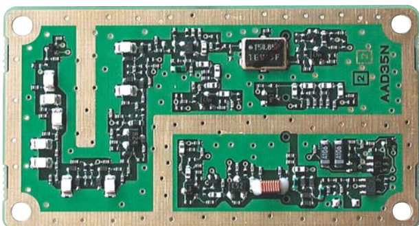
Multi Band Receiver Unit: SRX-1 for UHF, SRX-2 for VHF
